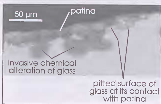
Figure 7. SEM image of a cross-sectional view of patina on glass (sample A2) showing invasive chemical alteration of the parent glass, and the pitted surface of glass at its contact with patina.
